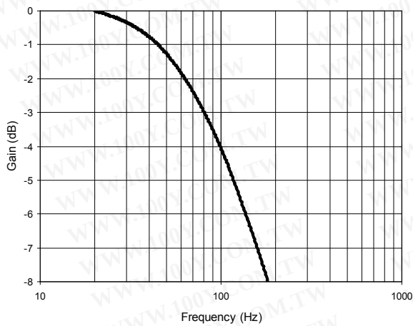
HAH1BV S/02 Frequency Bandwidth
